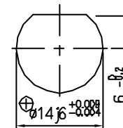
DETAIL OF SHAFRT END
