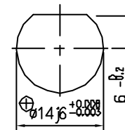
SHAFT EXTENSION
