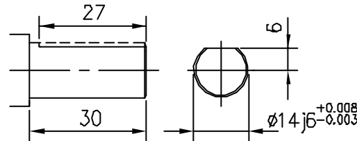
SHAFT EXTENSION
